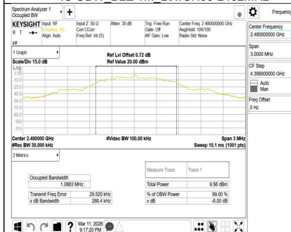
IC OBW_BLE 1M_HighCH39-2480MHz
