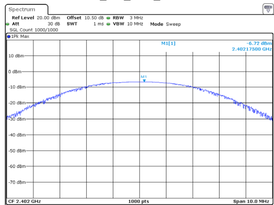
BLE_1M_Low_Channel
