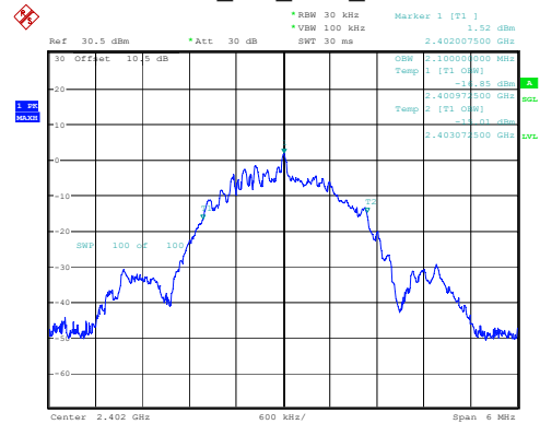
BLE_2M_Low_Channel
