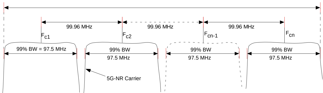
Figure 4.3.1.1 Carrier Aggregation
