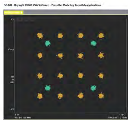
Sample 16QAM 27.6 GHz Vertical
