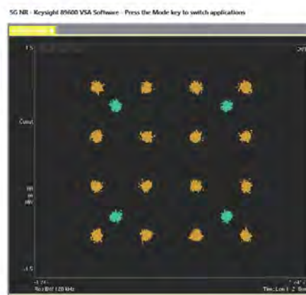
Sample 16QAM 27.6 GHz Horizontal
