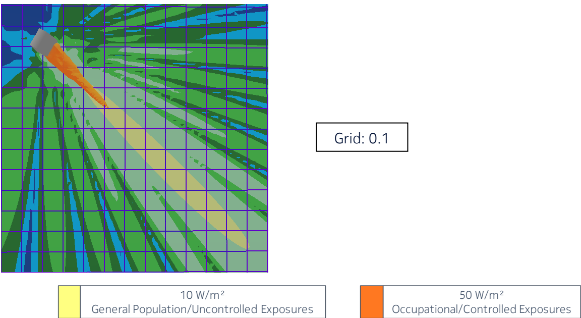
Figure 6 – Side view of the power density for the time-averaged actual maximum transmitted power of 0.283 W and the beam oriented in azimuth = 0° & elevation = +15°
