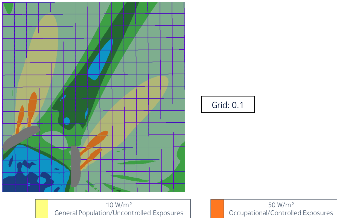
Figure 11 – Top view of the power density for the time-averaged maximum transmitted power of 1.13 W and the beam oriented in azimuth = -45°/+45° & elevation = 0°
