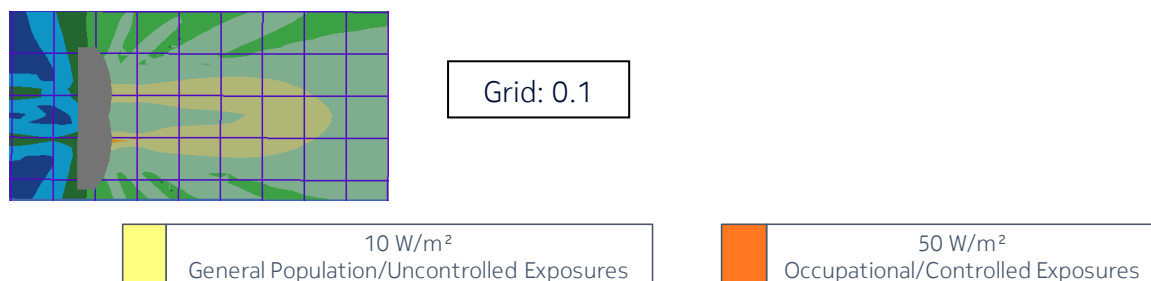
Figure 4 – Top view of the power density for the time-averaged actual maximum transmitted power of 0.283 W and the beam oriented in azimuth = 0° & elevation = 0°
