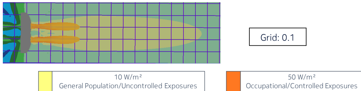
Figure 3 – Top view of the power density for the time-averaged maximum transmitted power of 1.13 W and the beam oriented in azimuth = 0° & elevation = 0°
