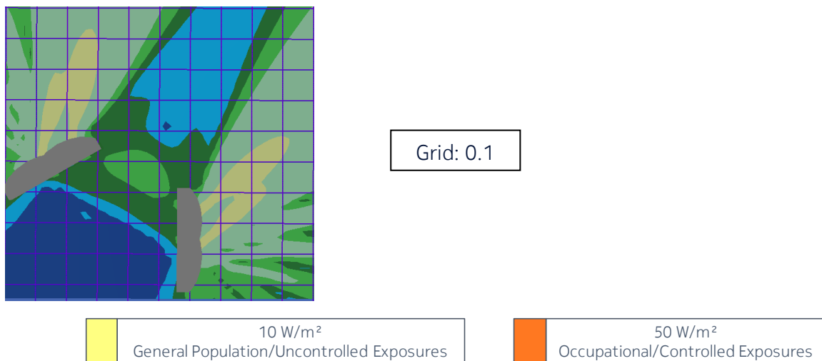
Figure 12 – Top view of the power density for the time-averaged actual maximum transmitted power of 0.283 W and the beam oriented in azimuth = -45°/+45° & elevation = 0°
