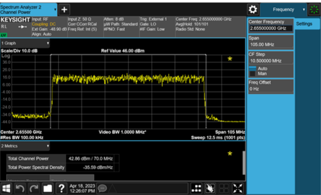
TM 3.1a, 256QAM, CF 2655 MHz, TX4
