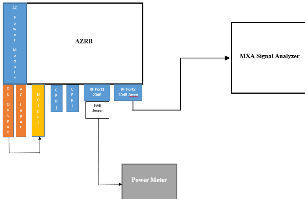
Figure 1. Setup Diagram of Conducted Test
