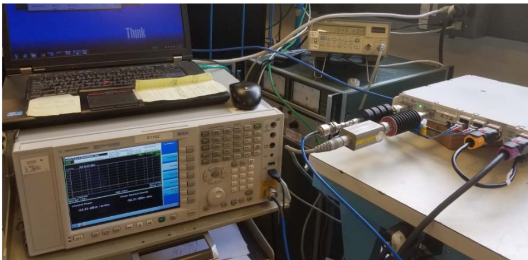
Figure 3. Setup Diagram of Conducted Test
