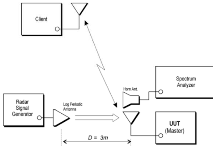
Figure 3. Setup Diagram of DFS Test
