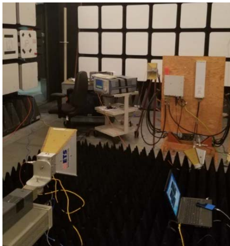
Figure 6. Setup Photos of DFS Test of AZRB with PAS2457-CC1 Antenna
