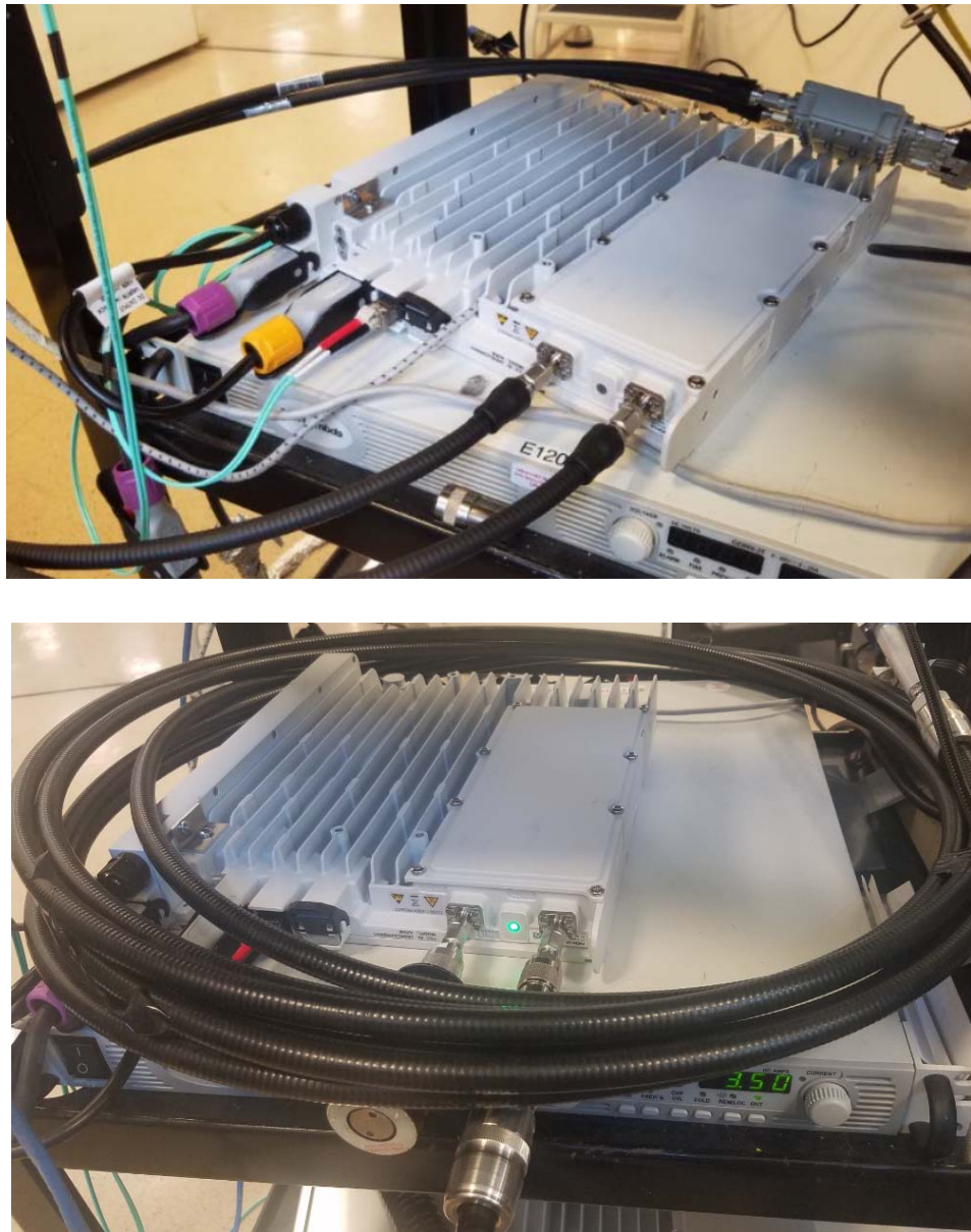
Figure 4. Setup Diagram of Conducted Test
