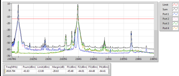
64QAM-2628.8-1RB high+2648.6-1RB low
