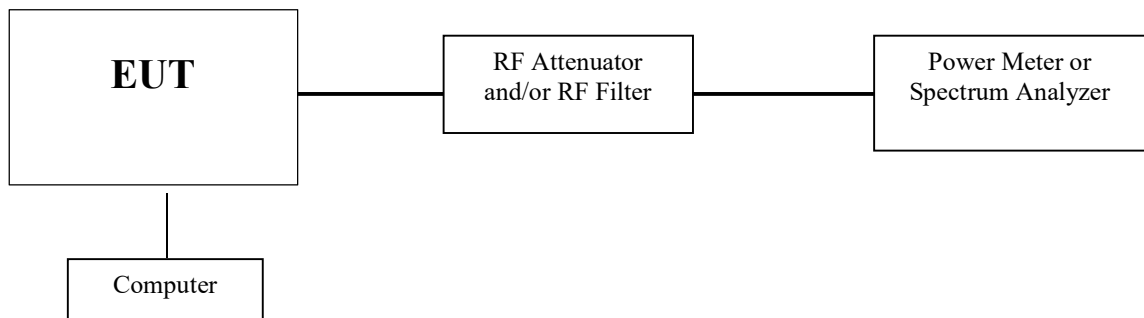
Figure 1. Setup Diagram of Conducted Test for RF Output Power, Power Spectrum Density, Occupied Bandwidth and Unwanted Emissions.
