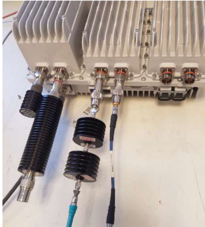
Figure 4. Photo of RF Conducted Tests
