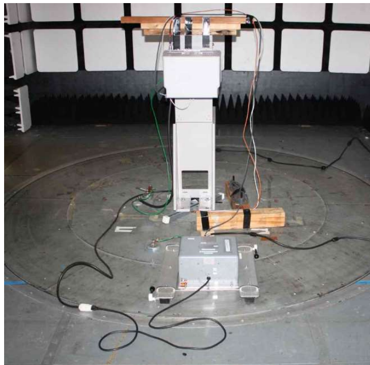
Figure 7. Photo of AC Power Line Conducted Test
