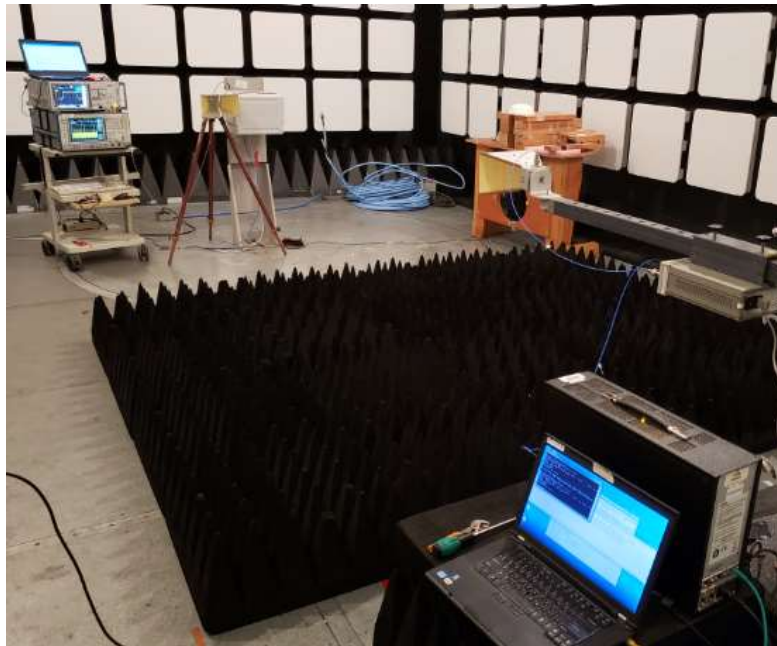
Figure 6. Photos of DFS Tests
