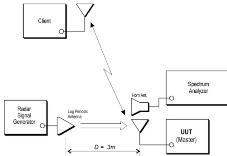
Figure 3. The Setup Diagram of DFS Test
