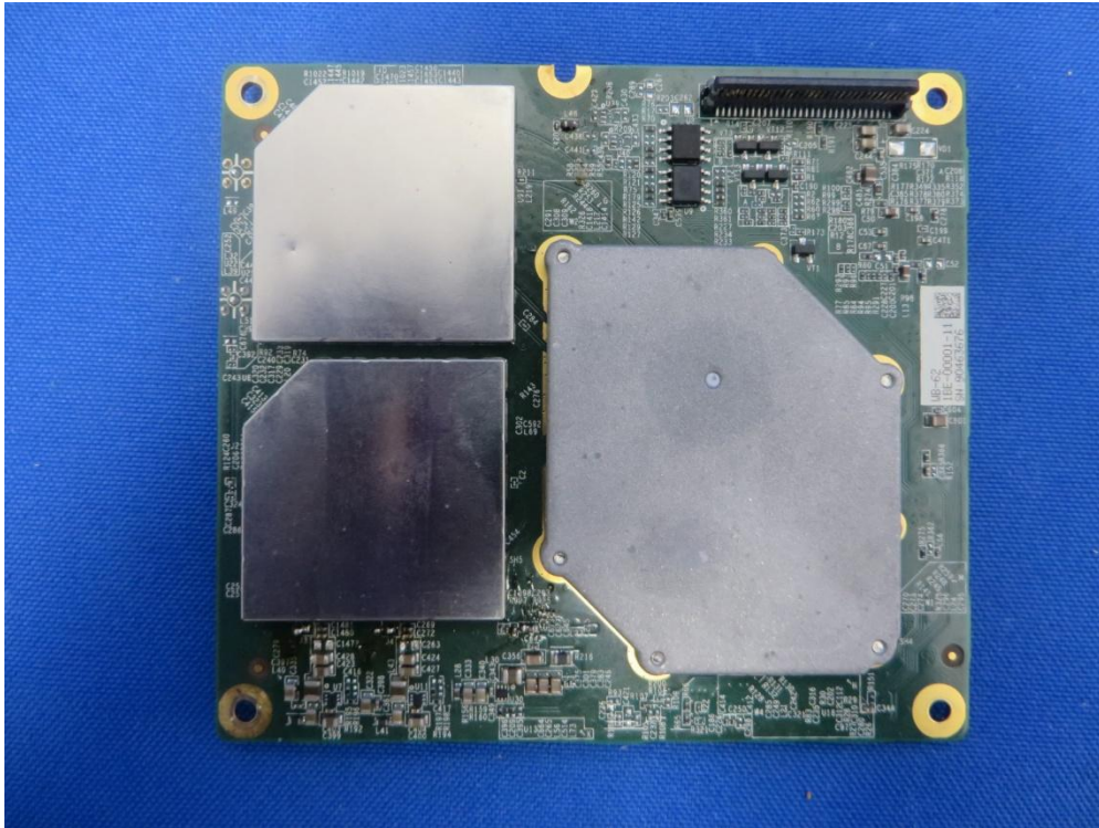
(7) Module Photo (WiFi RF Board Top View with Shields Installed)
