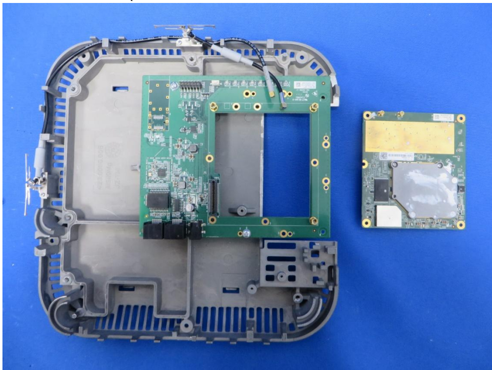
(2) Test Fixture Photo (Shown with WiFi RF Board and Interface Board Removed)
