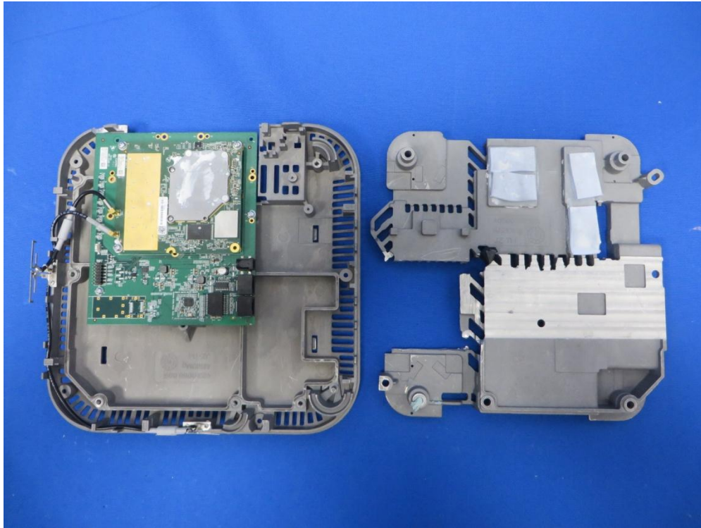
(1) Test Fixture Photo (Cover Removed)
