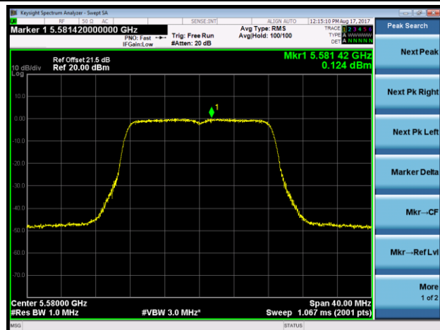
Channel 116 (5580MHz)
