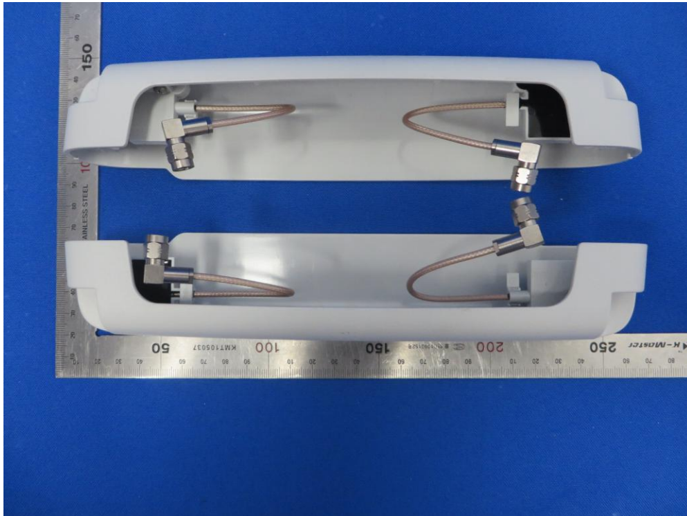
(7) Antenna Photo (Galtronics Small Omni Antenna)
