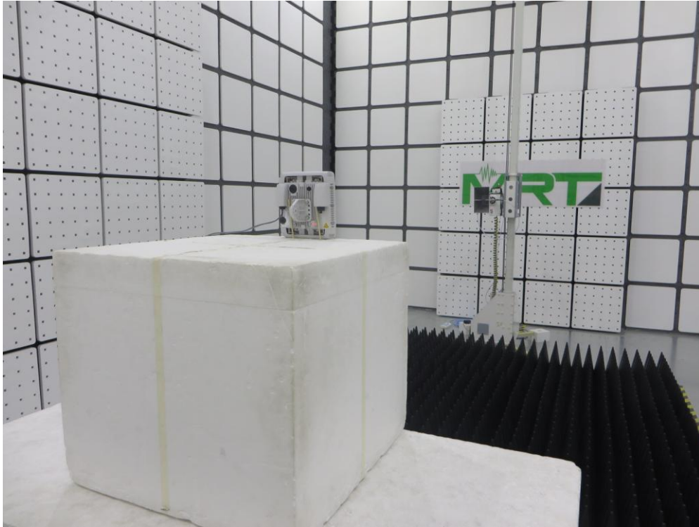
Description: Galtronics Small Omni Antenna Radiated Emission Test Setup for 18GHz ~ 40GHz
