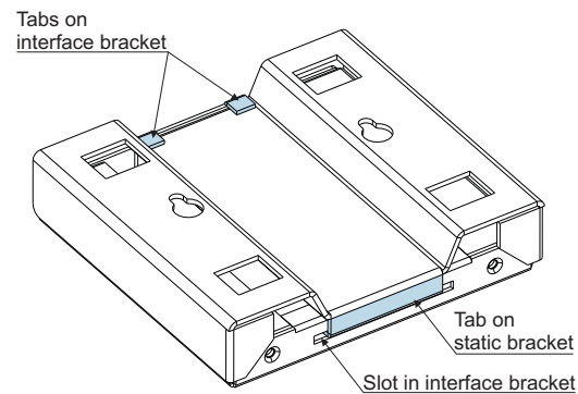
Figure 18 Correct bracket alignment
