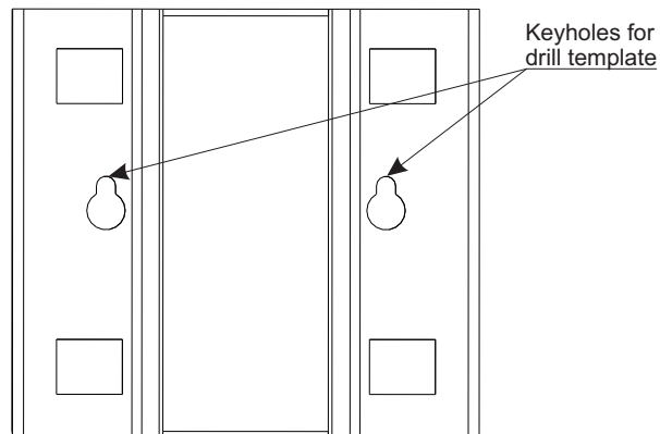
Figure 6 Drilling the holes
