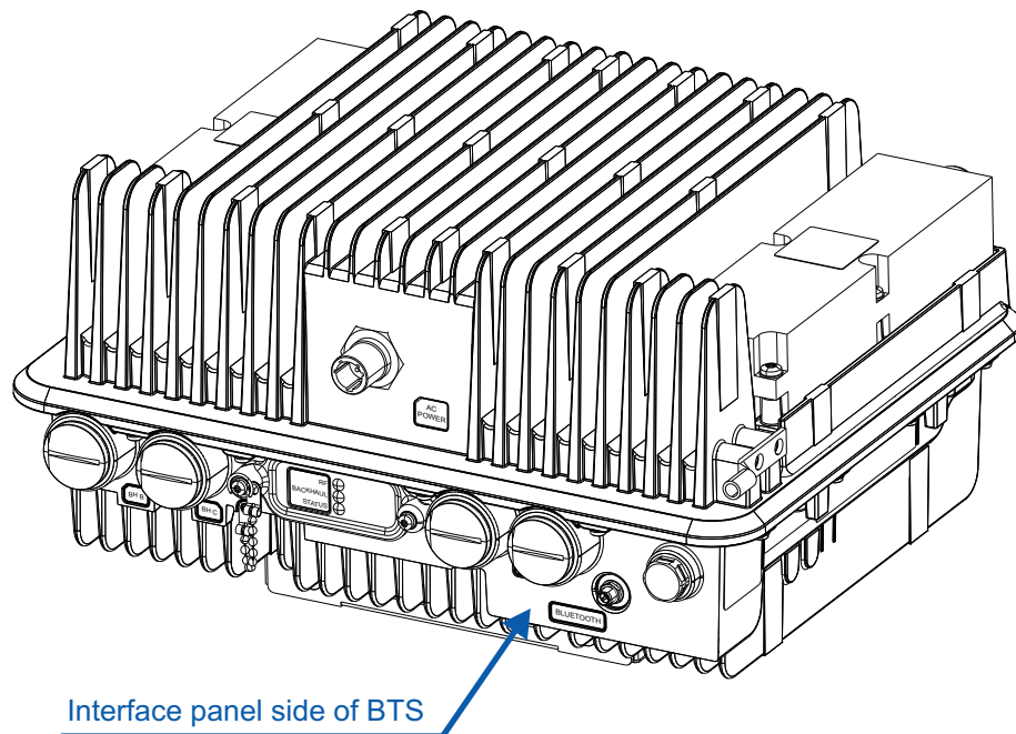
Figure 1 Flexi Zone Micro BTS (FWHR) interface panel
