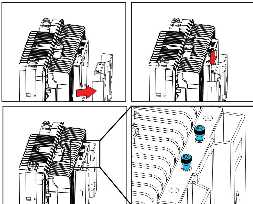
Figure 10 Installing the BTS on a wall
