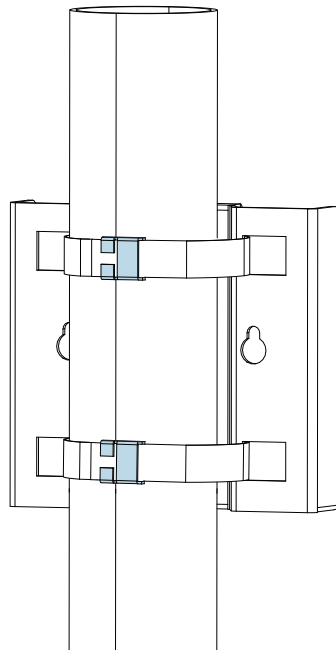
Figure 16 Installing the installation plate to the pole
