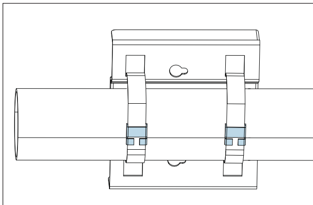
Figure 25 Installing the static mounting bracket on the pole
