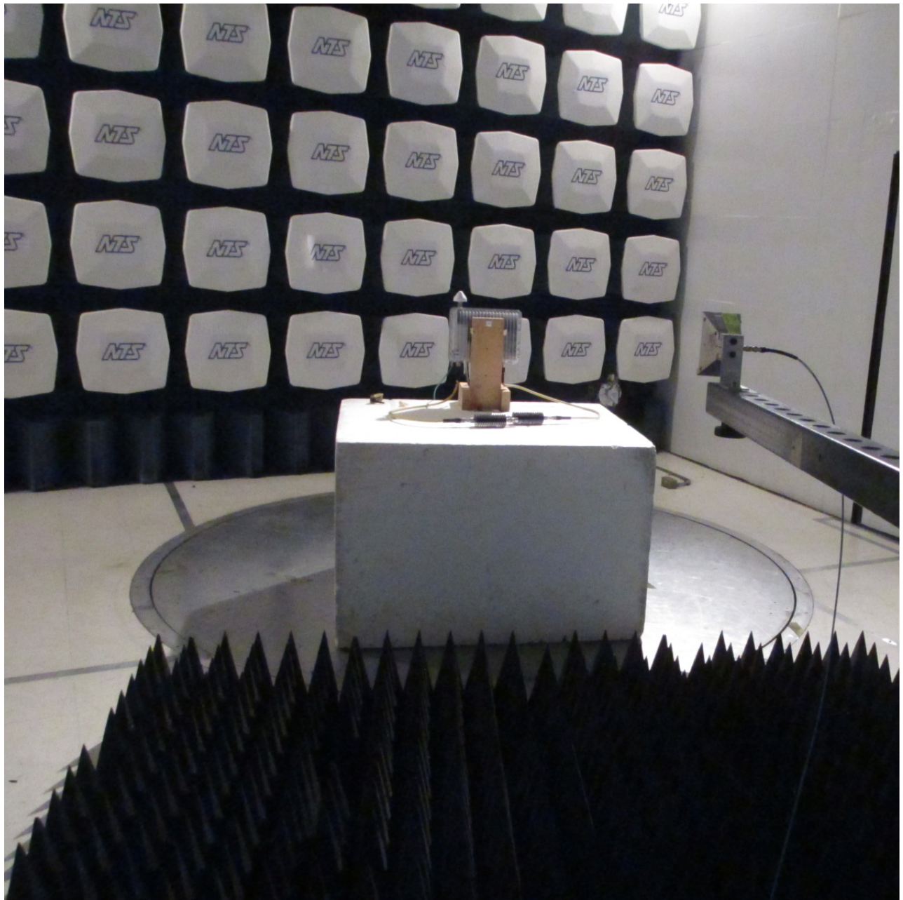
Radiated Emissions Setup – 18GHz to 27GHz
