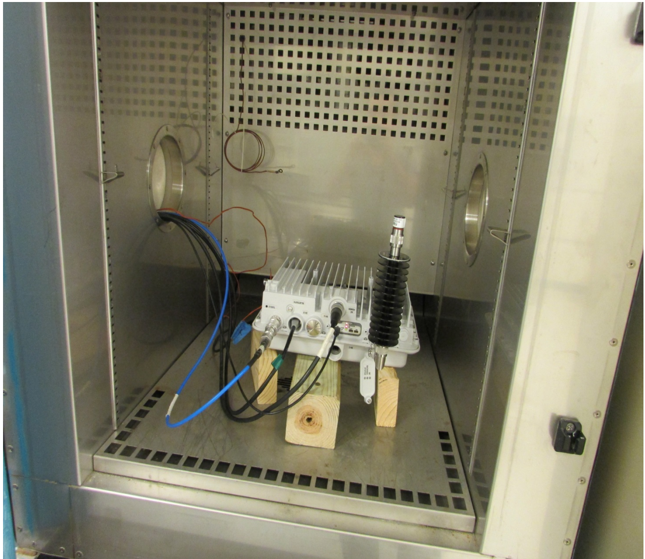
Frequency Stability Setup
