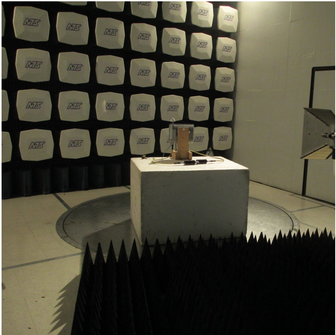
Radiated Emissions Setup – 1GHz to 18GHz
