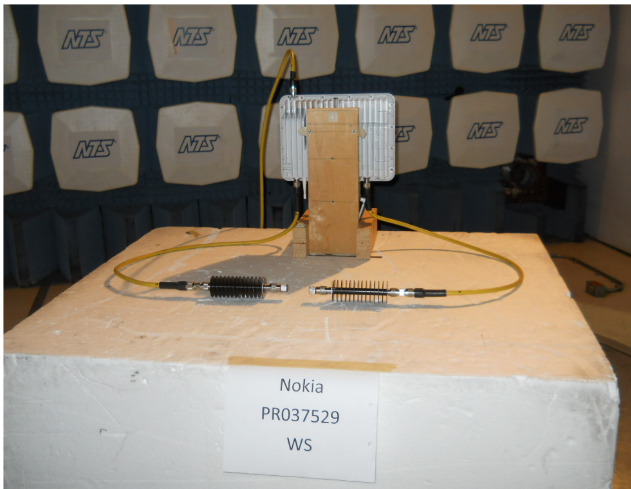
Radiated Emissions Setup
