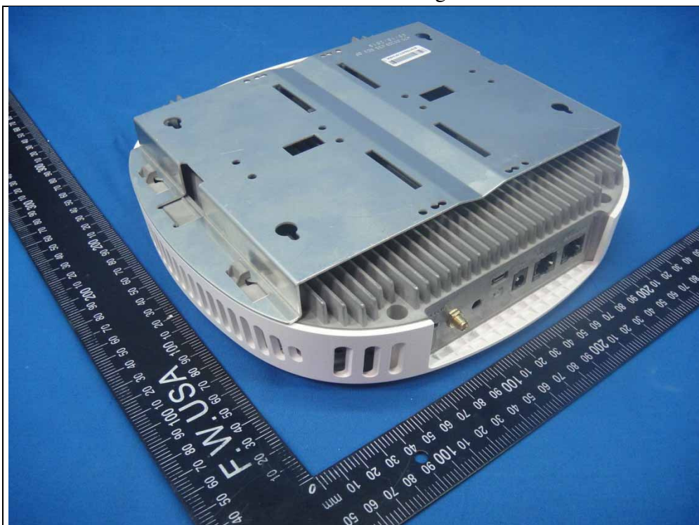
FZP bottom with shielding cover
