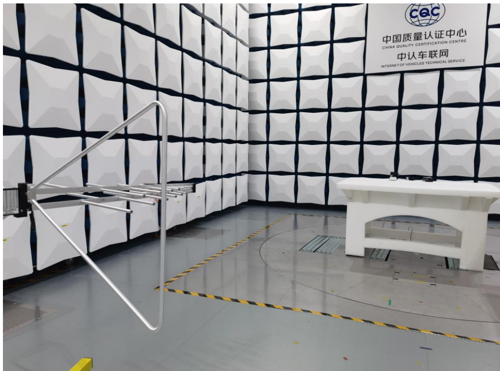
30MHz-1GHz
