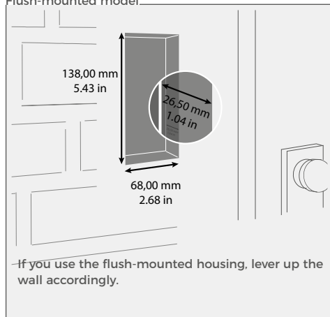
Flush-mounted model
