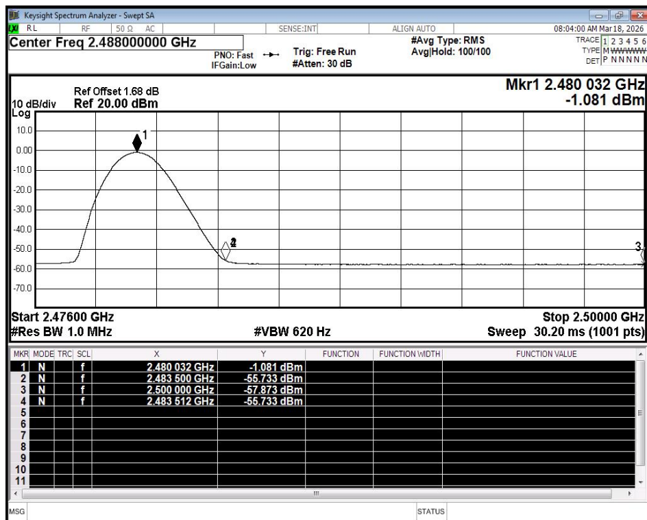
Restrict Band NVNT BLE 2480MHz Ant1 Average
