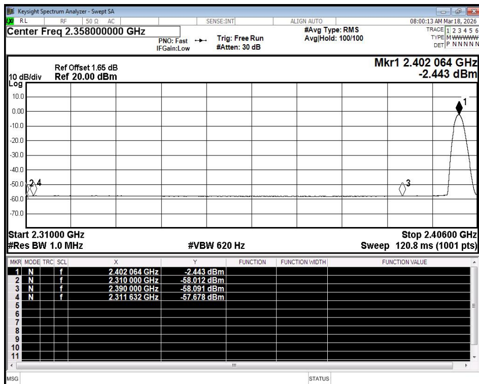
Restrict Band NVNT BLE 2402MHz Ant1 Average
