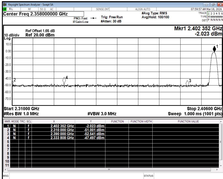
Restrict Band NVNT BLE 2402MHz Ant1 Peak
