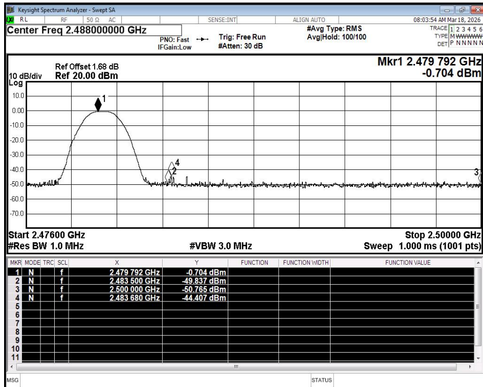
Restrict Band NVNT BLE 2480MHz Ant1 Peak
