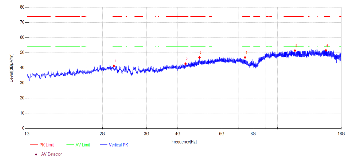
Test Graph
