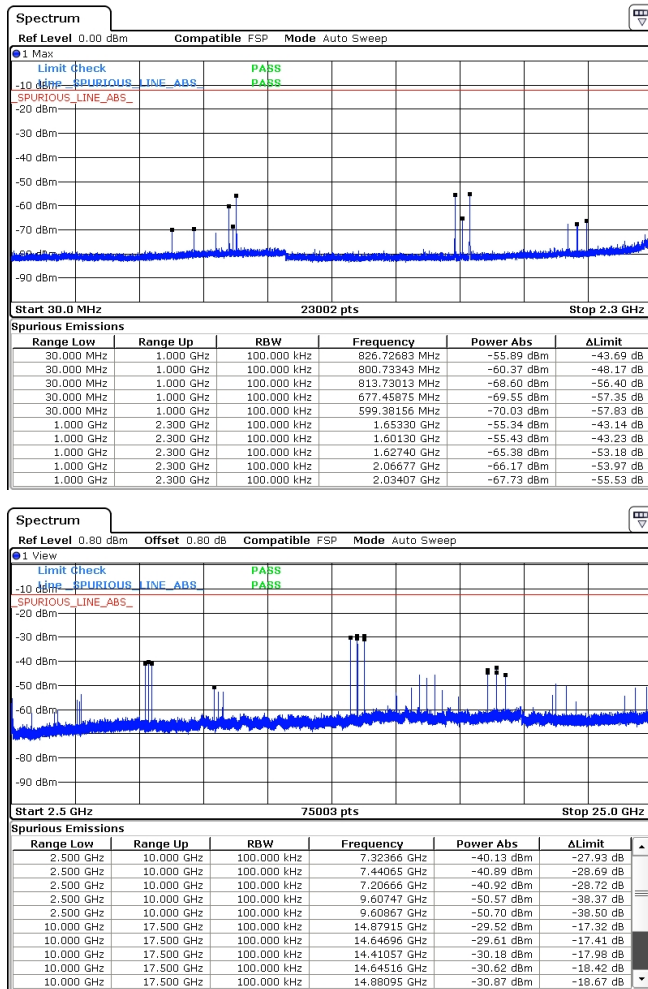
Figure 9(b): Conducted Transmitter Emissions Measured.
