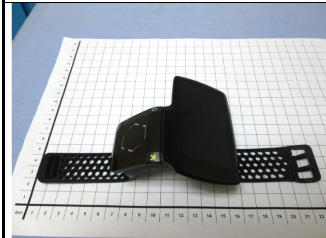
EUT with Battery 3
