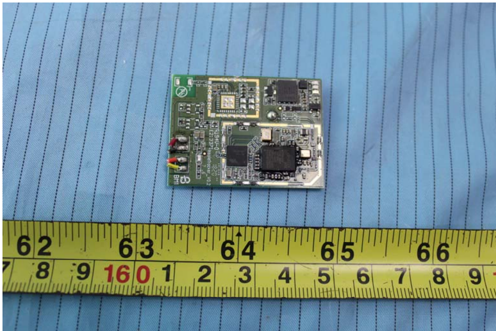
EUT – Main PCB shielding off Bottom View
