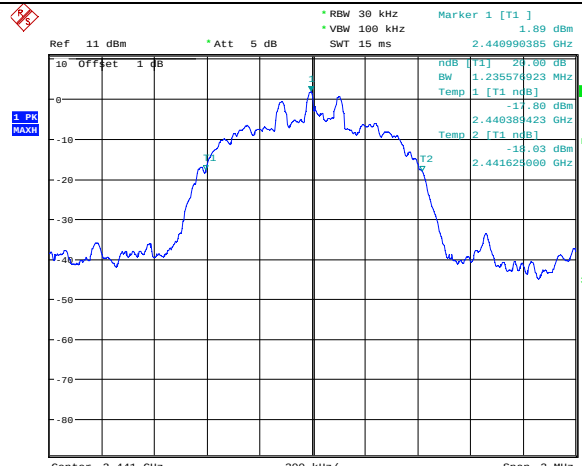
8-DPSK Mode 2441MHz
