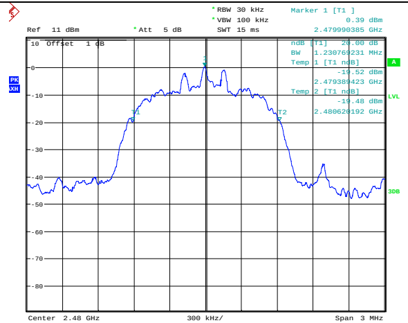
8-DPSK Mode 2480MHz
