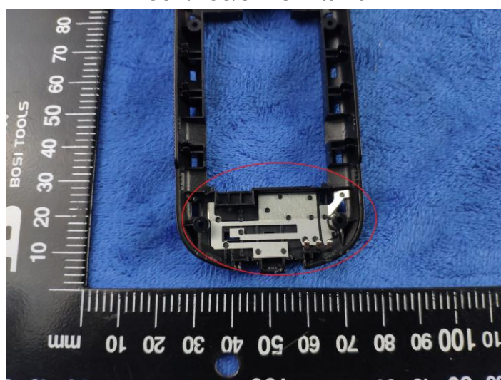
GSM/PCS/UMTS Antenna
