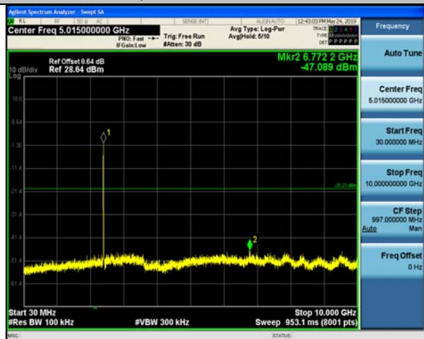
Spurious emission
