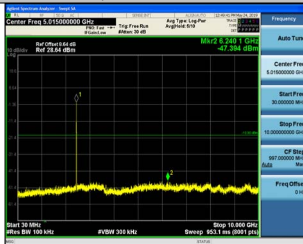
Spurious emission
