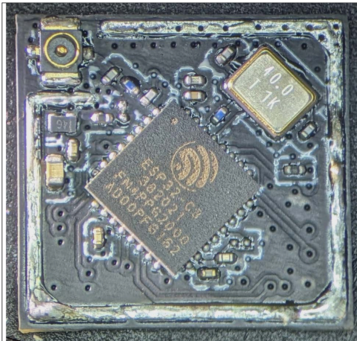
Module Top – Shield Removed
