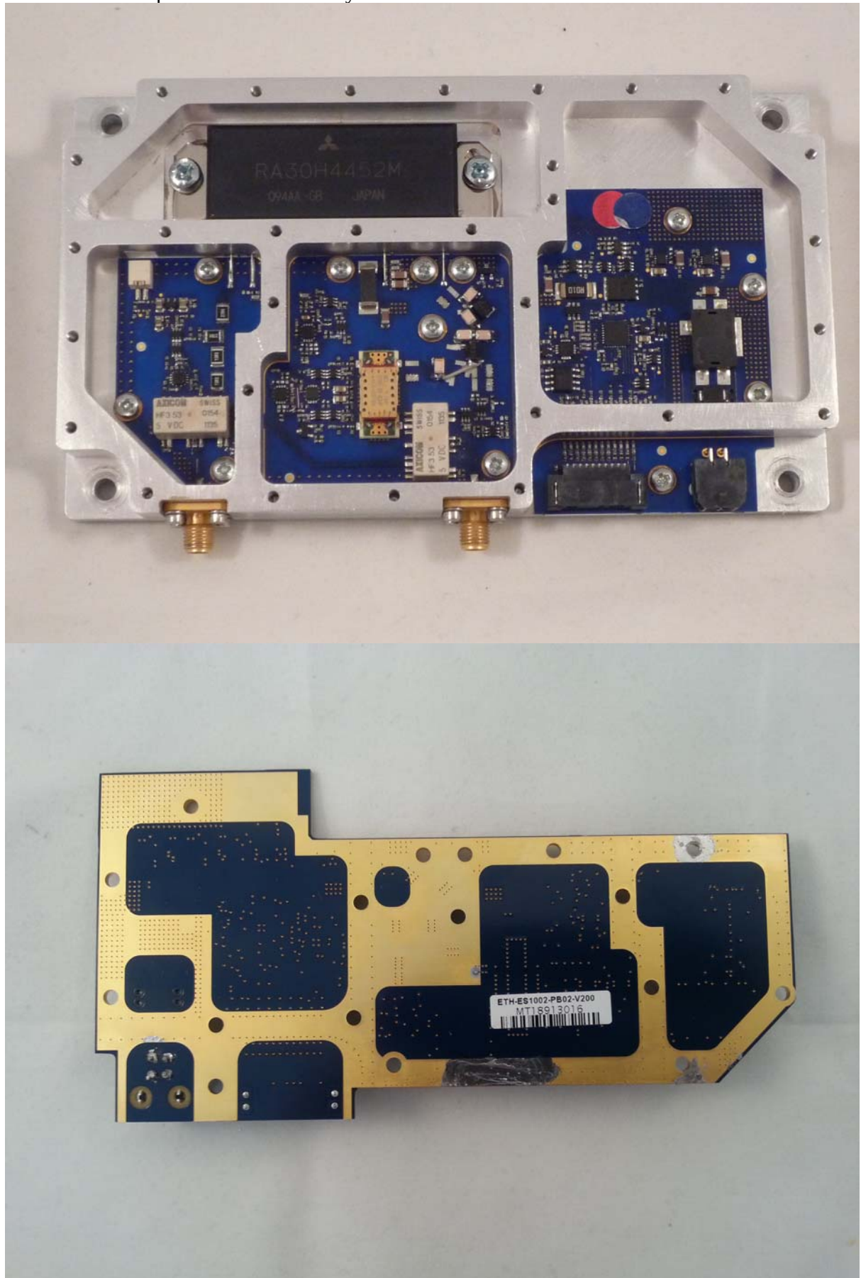
PB02 Power Amplifier PCB Assembly
