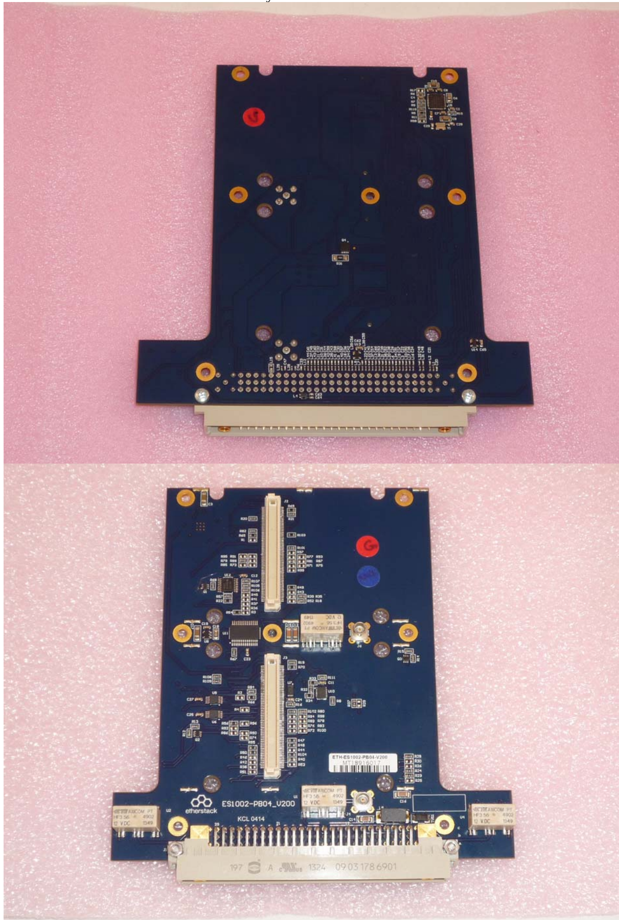
PB04 Transceiver Carrier PCB Assembly
