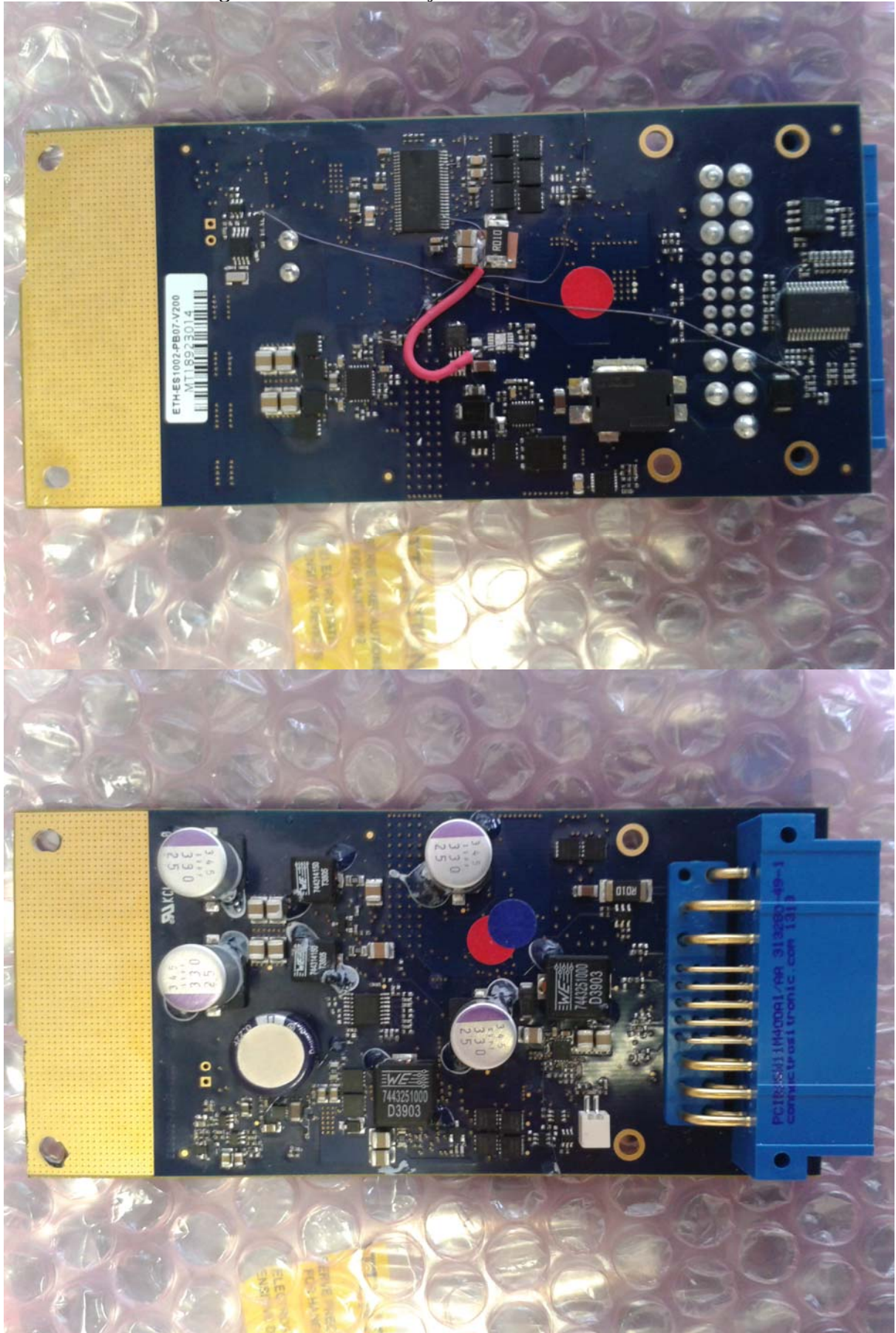
PB07 DC Power Management PCB Assembly
