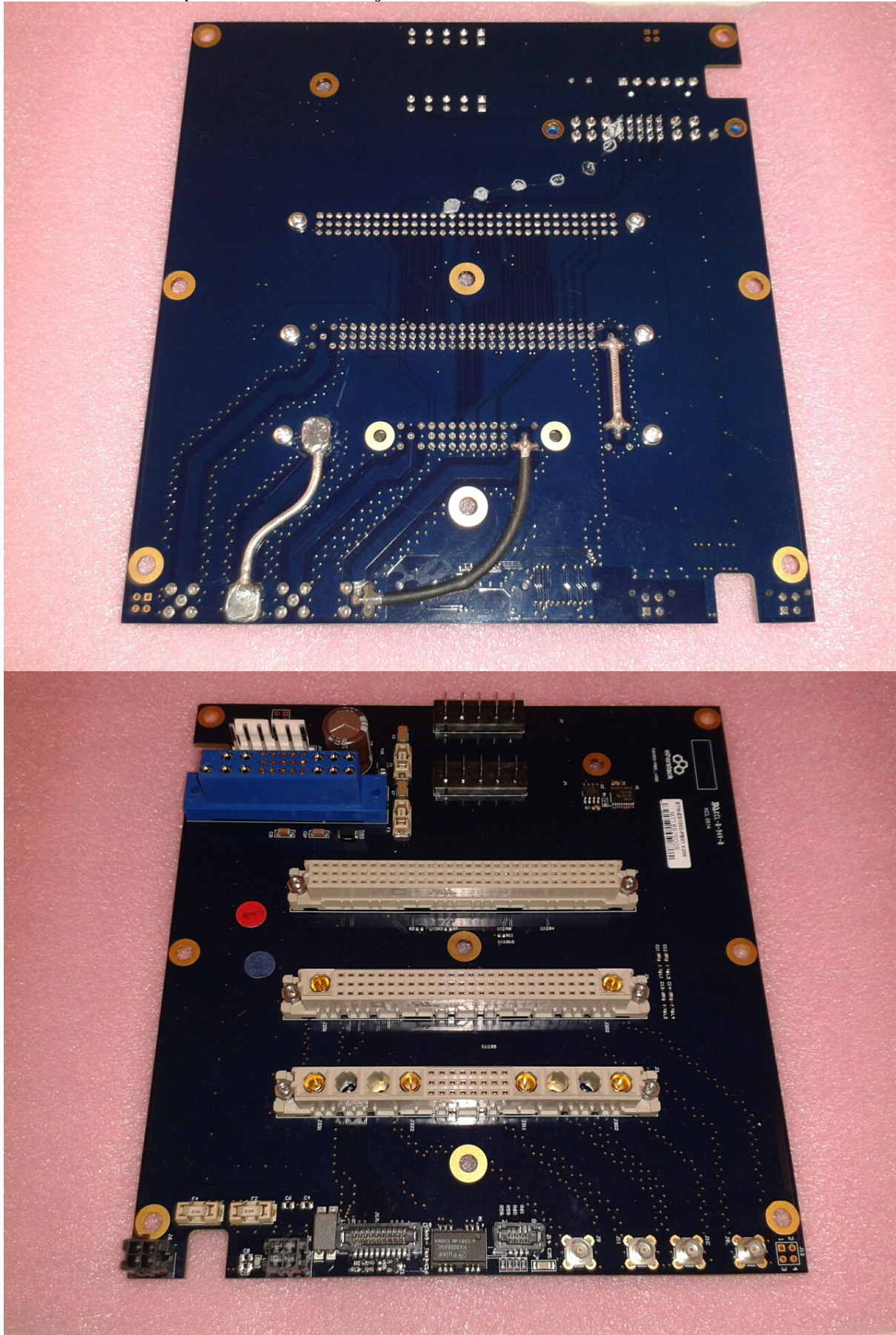
Main Chassis Backplane PCB Assembly
