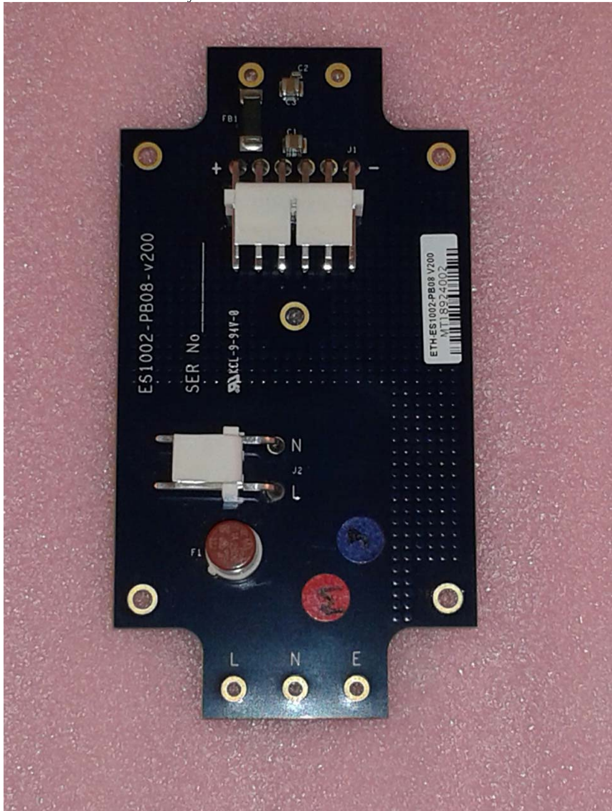
PB08 AC-DC PCB Assembly
