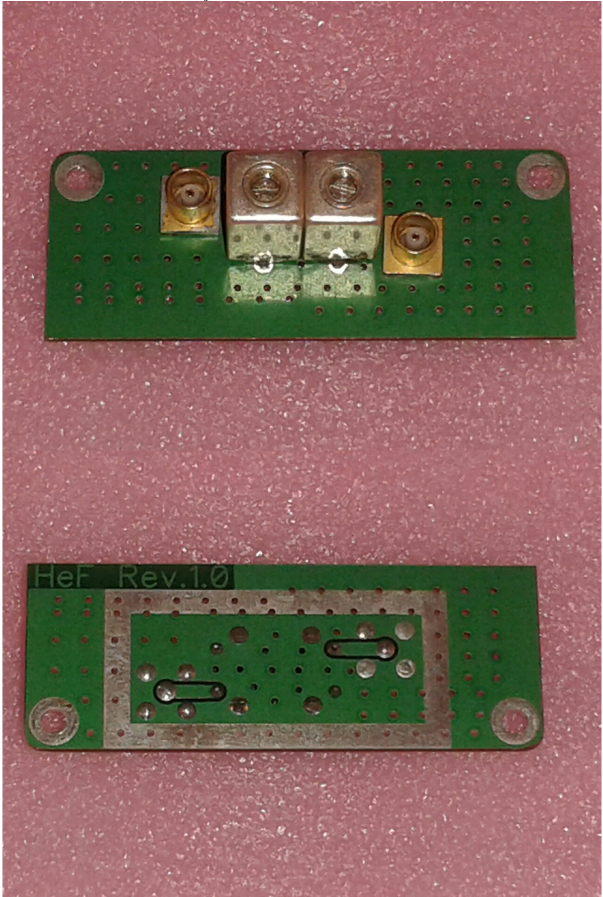
PB09 UHF Filter PCB Assembly
