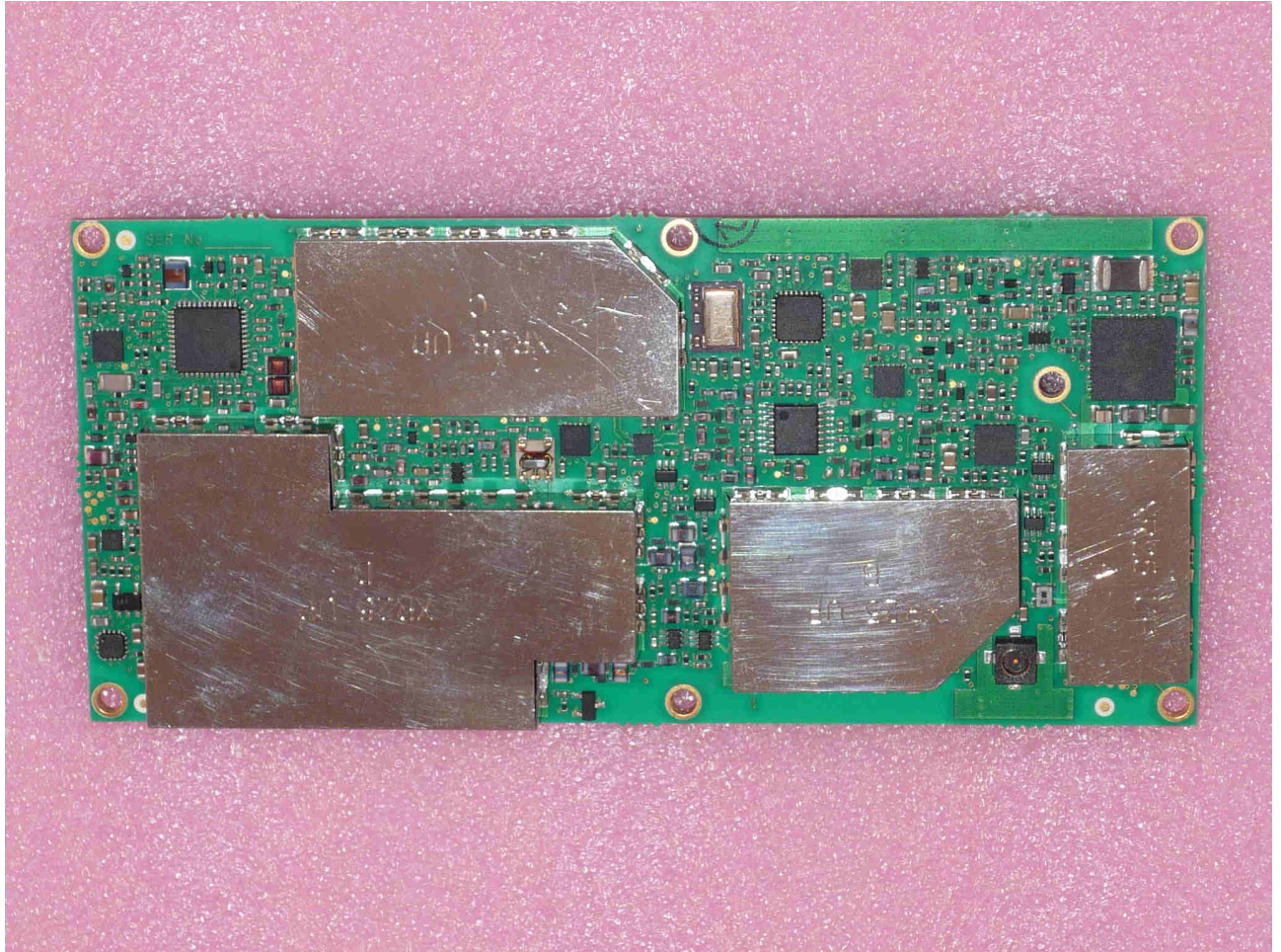
XR25 UHF Transceiver Top with Shields
