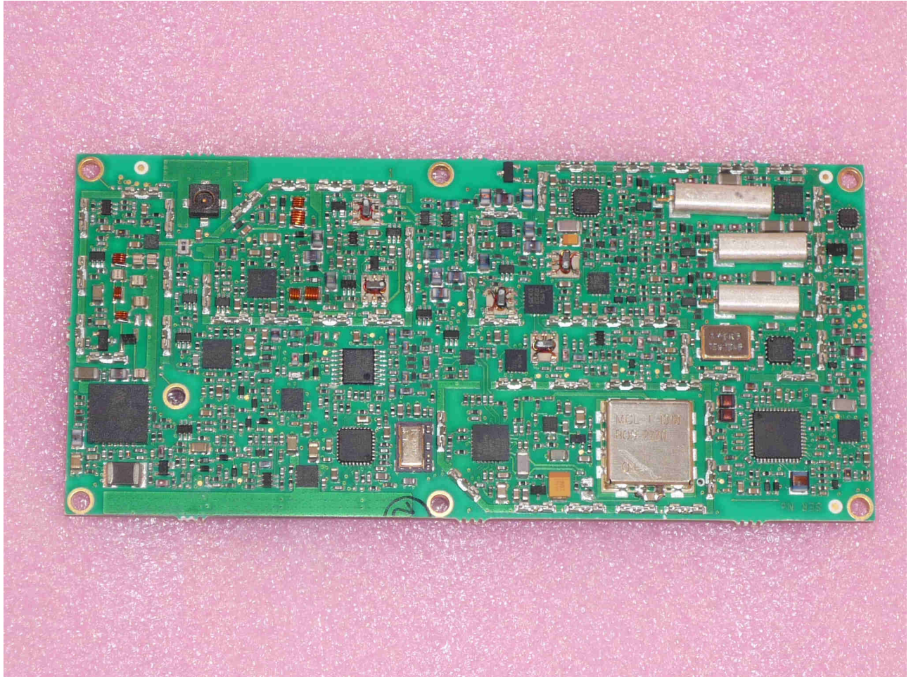
XR25 UHF Transceiver Top without Shields
