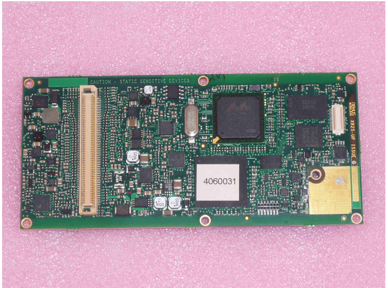
XR25 UHF Transceiver Bottom
