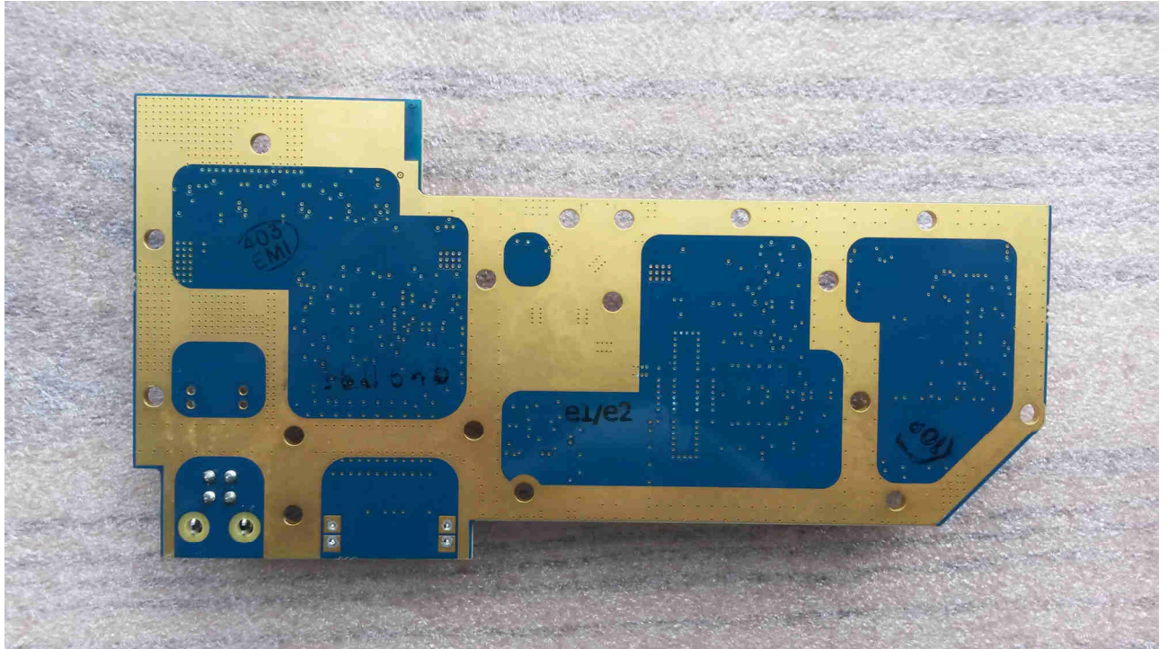
ES1002-PB02 UHF High Power Amplifier PCB Assembly Bottom
