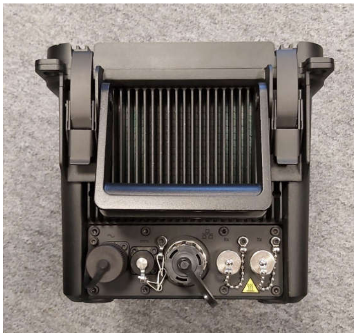
Photo 7 Two External RF Ports and No Internal Duplexer (Configuration 2) – Front Panel with Two external RF Ports.
