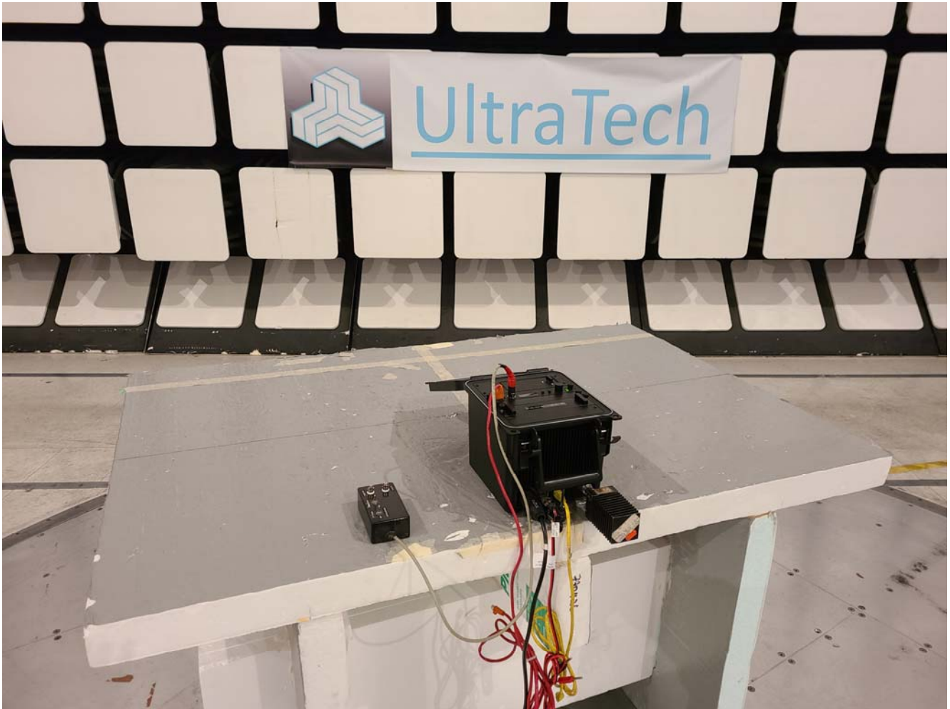
Test Configuration 1 Radiated Emissions at 3 m, 30 - 1000 MHz
