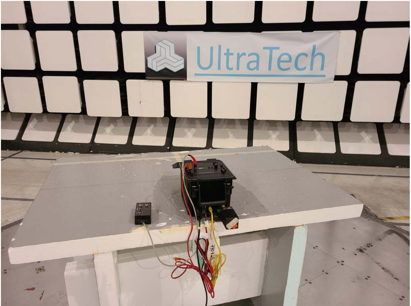
Test Configuration 2 or 3 Radiated Emissions at 3 m, 30 - 1000 MHz
