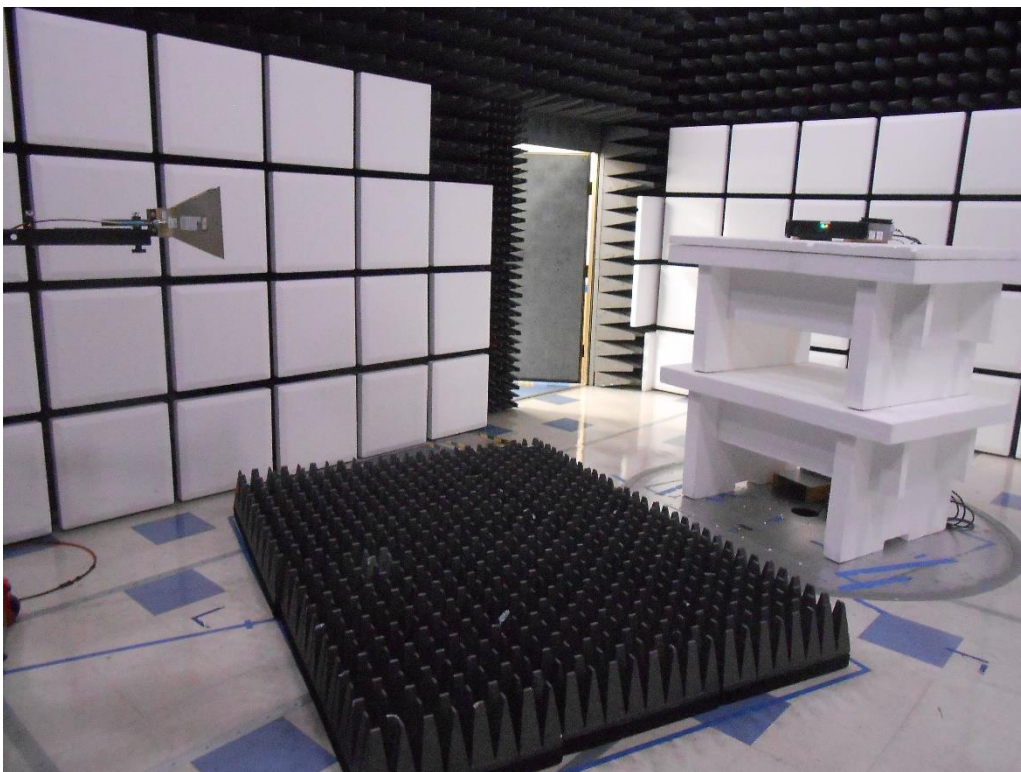
Radiated RF
