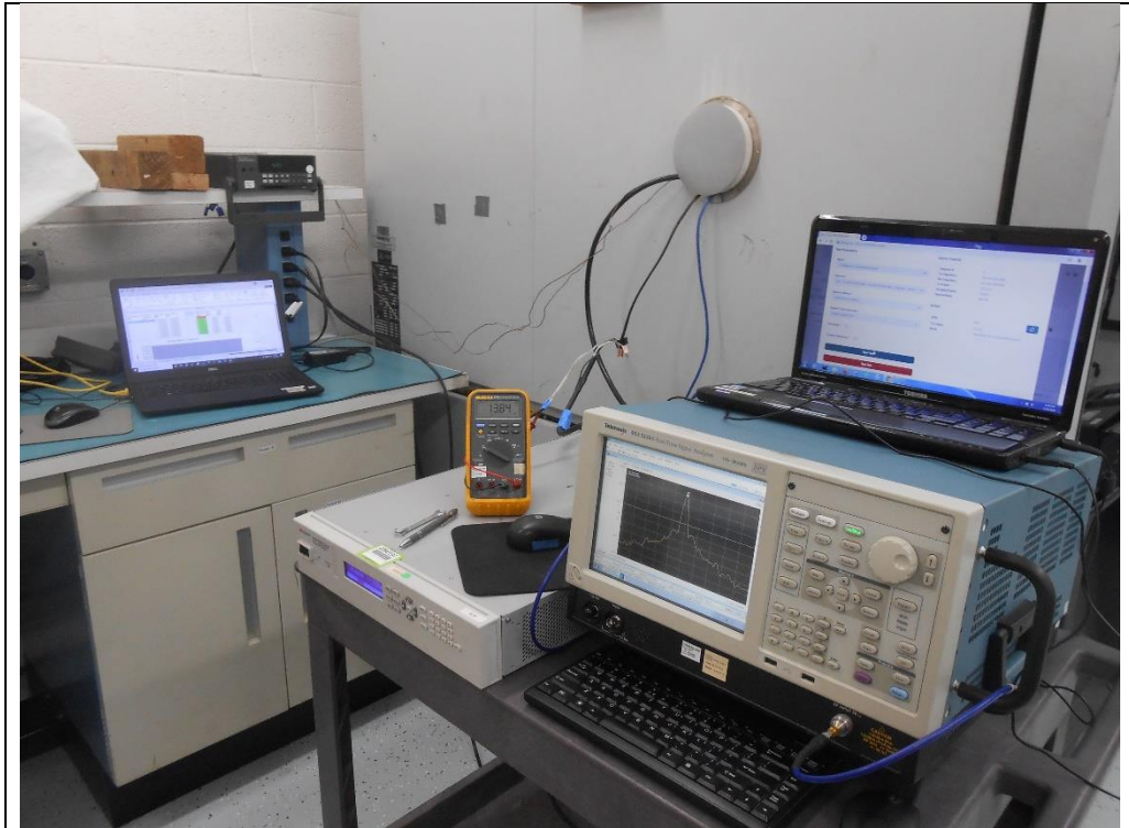
Frequency Stability #2
