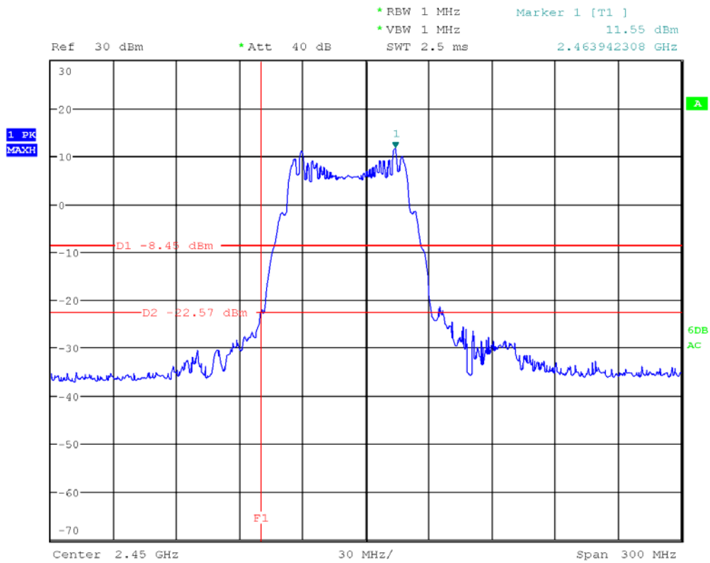
Graph 3: Lower band-edge emissions
