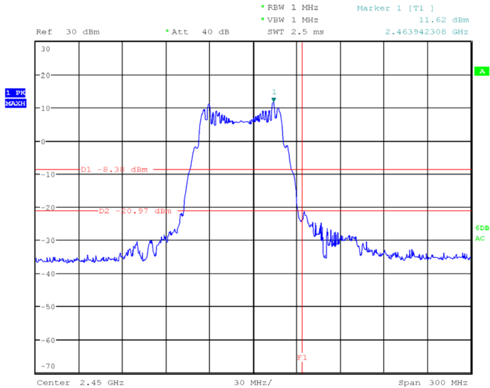
Graph 4: Upper band-edge emissions
