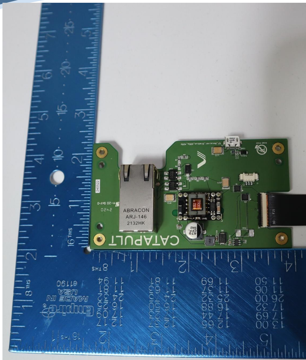
Network PCB
