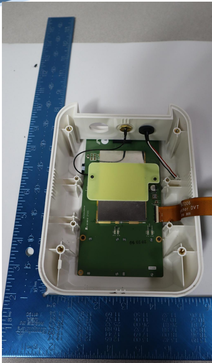
Top Internal Main pcb
