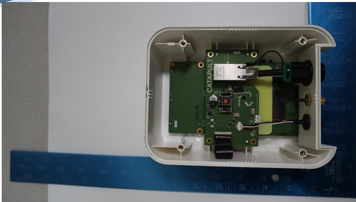
Internal Top
