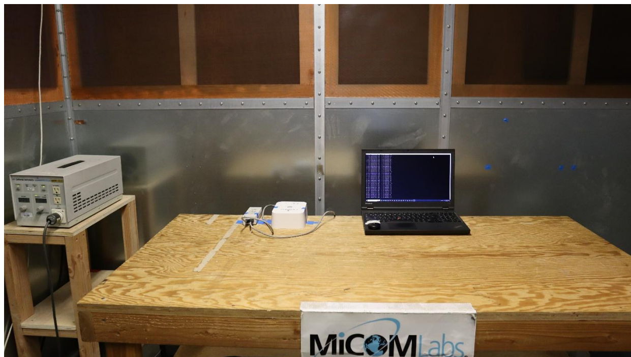
AC wireline test setup, Front View
