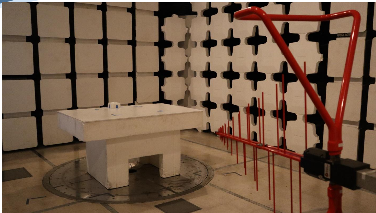
Radiated Digital Emissions 30MHz-1GHz Vertical Test Setup
