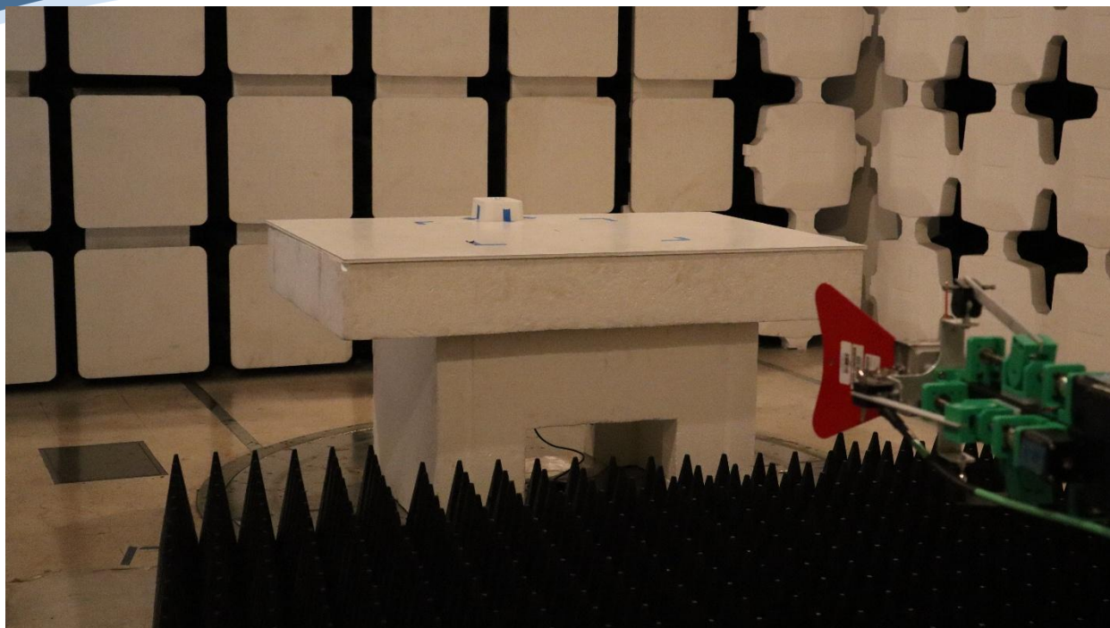
Radiated Digital Emissions Above 1GHz Horizontal Test Setup
