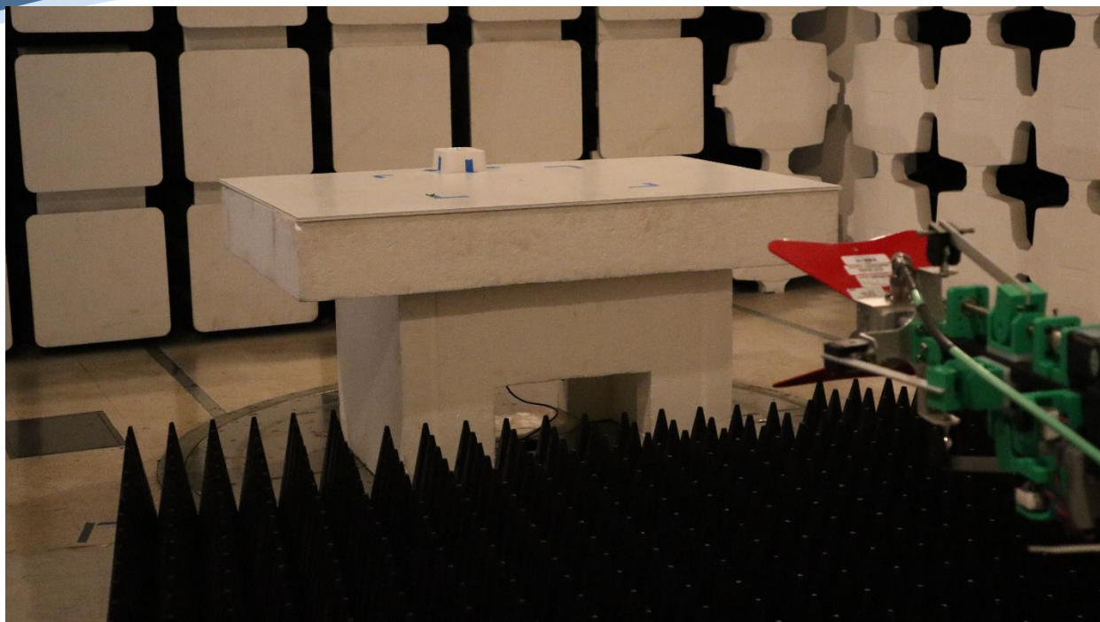
Radiated Digital Emissions Above 1GHz Vertical Test Setup
