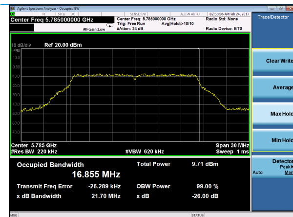
Mid Channel – 802.11a HT-20
