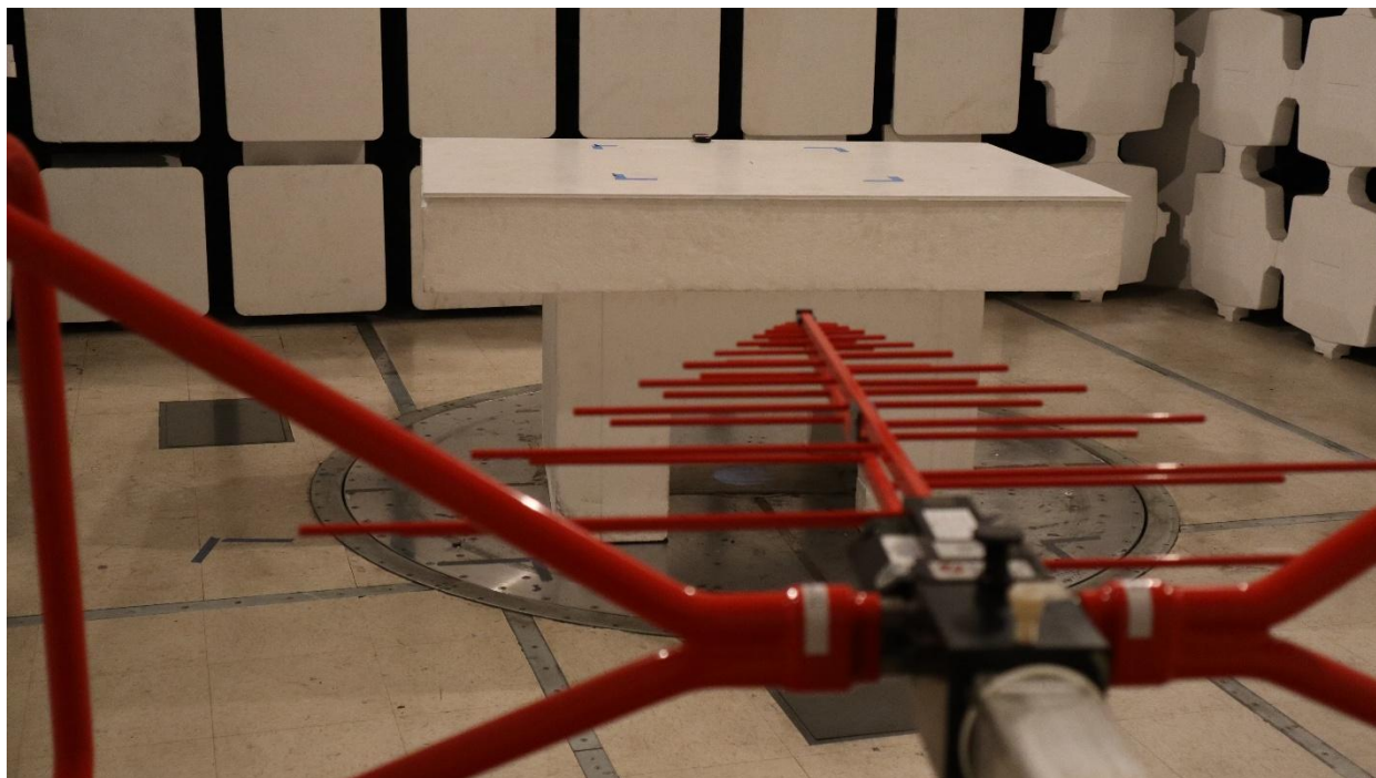
Radiated Emissions 30MHz-1GHz Test Setup
