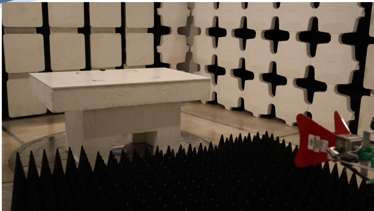
Radiated Emissions 1-18GHz Test Setup
