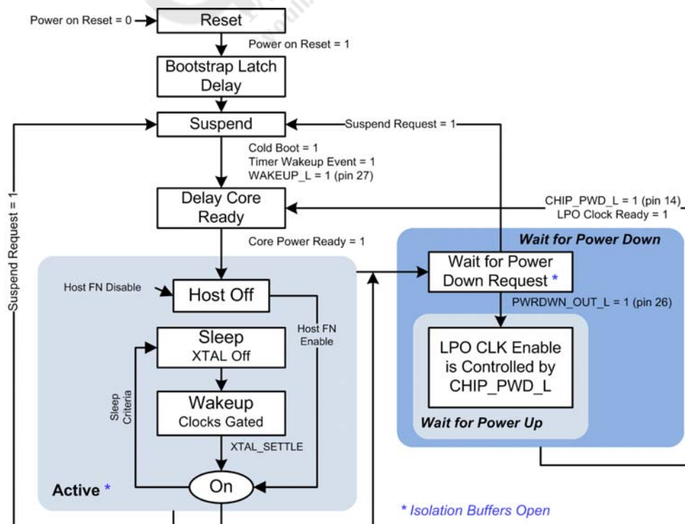
Figure 2-1 Wakeup Manager
