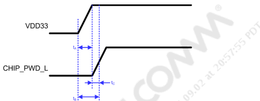
Figure 4-4 Power-On-Reset Timing
