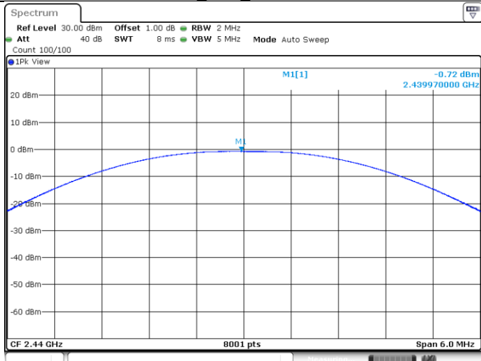
BLE_Ant1_2440MHz
