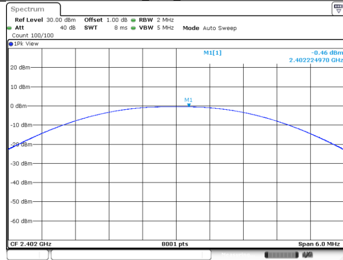
BLE_Ant1_2402MHz
