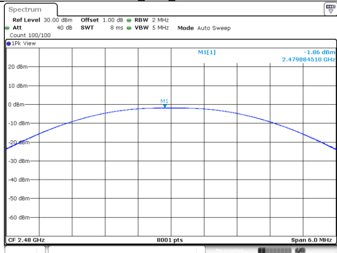
BLE_Ant1_2480MHz
