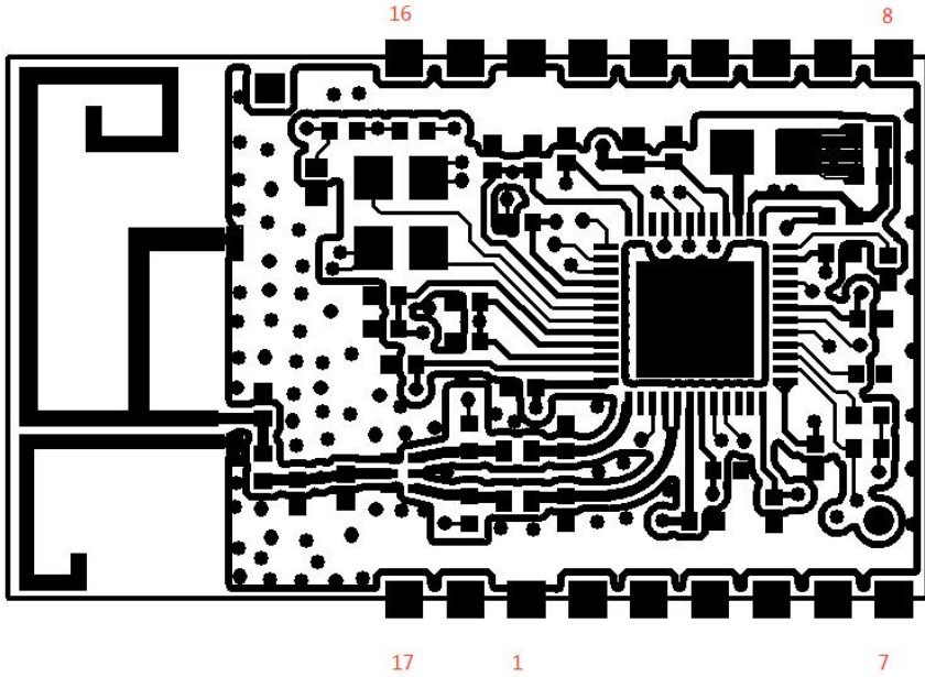
Figure2. Pin Definition
