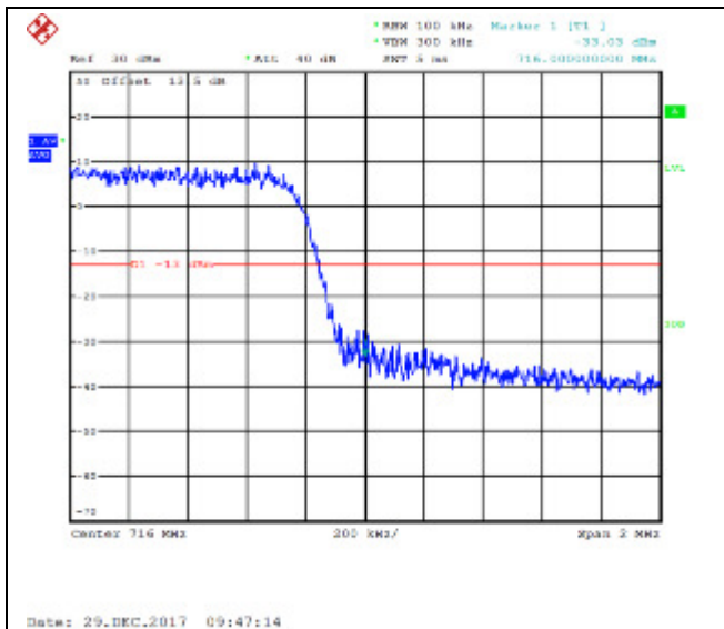
QPSK High channel-12 RB offset 13
