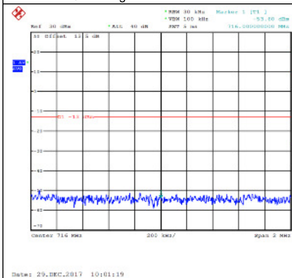
QPSK High channel-1 RB offset 24
