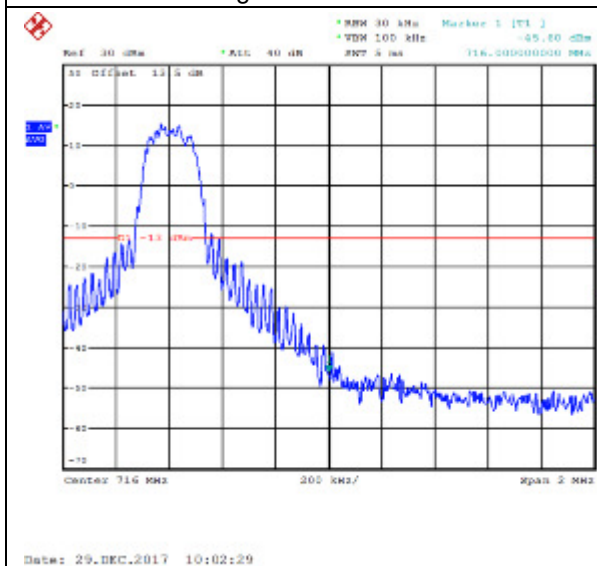
QPSK High channel-1 RB offset 49
