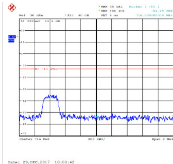
16QAM High channel-1 RB offset 0
