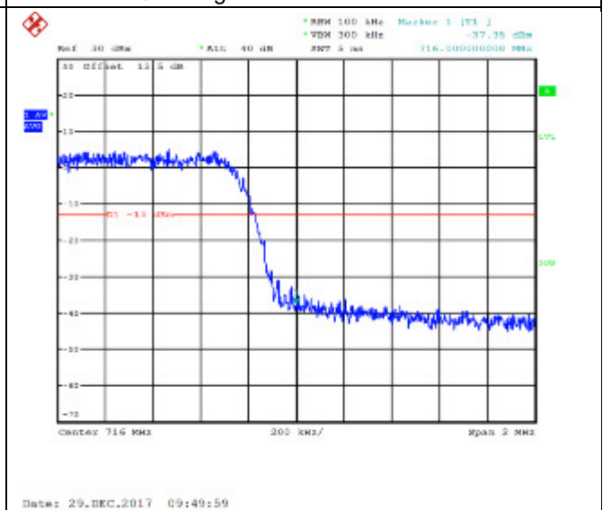
16QAM High channel-25 RB offset 0
