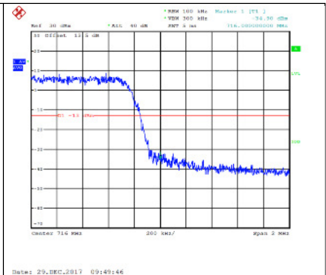
16QAM High channel-12 RB offset 13
