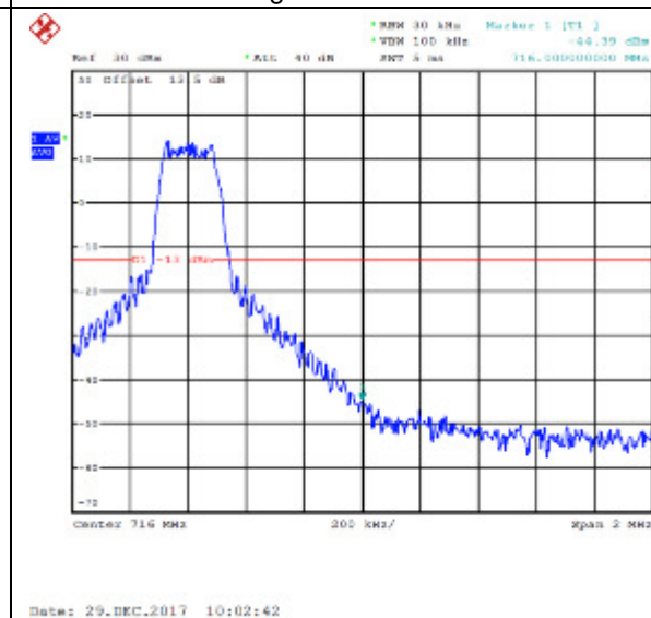
16QAM High channel-1 RB offset 49
