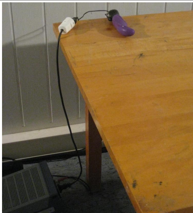
Test Setup : Conducted Emissions
