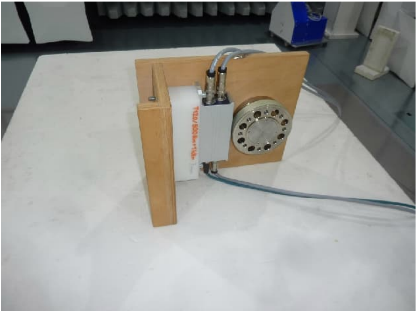
BG 3 _ Test setup semi anechoic chamber (position 3)
