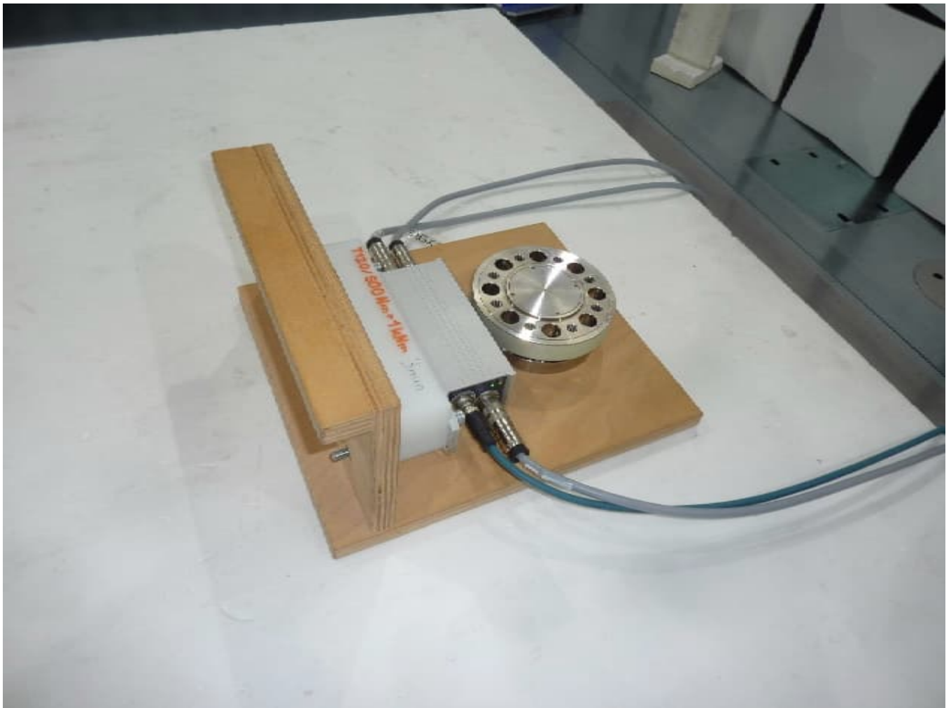
BG3_ Test setup semi anechoic chamber (position 2)
