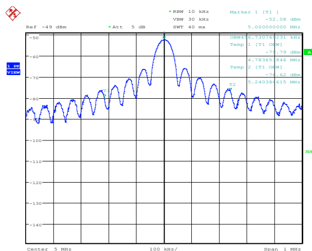
Plot T10F S3 carrier 5 MHz
