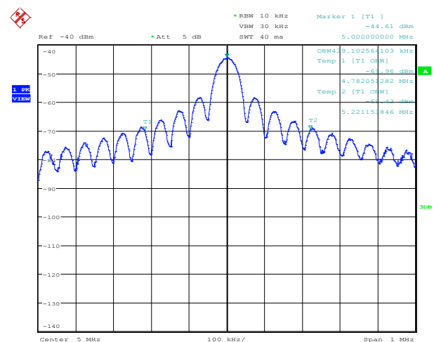
Plot T10F S2 carrier 5 MHz
