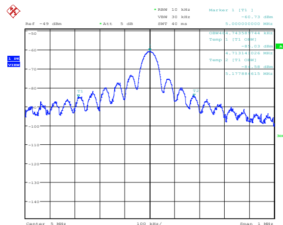
Plot T10F S6 carrier 5 MHz
