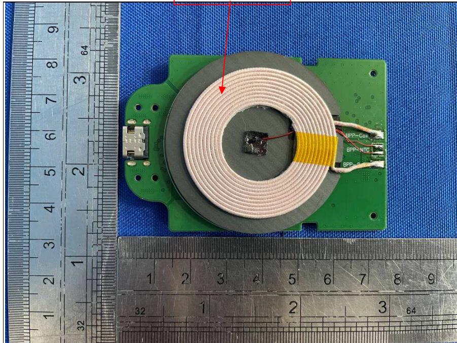
BPP5W Coil
