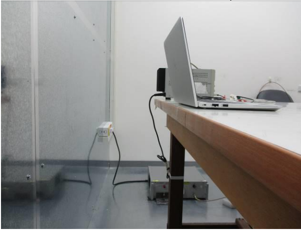
FCC_15_247_BLE_Conduction_Setup
