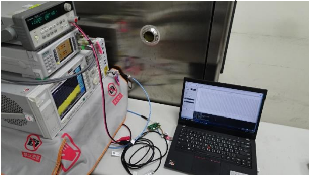
FCC_15_247_BLE_Radiated_Setup
