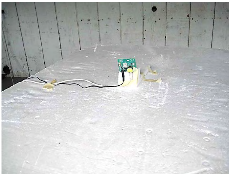
Radiated Spurious Emissions, 9kHz-40GHz Overall Test Setup
