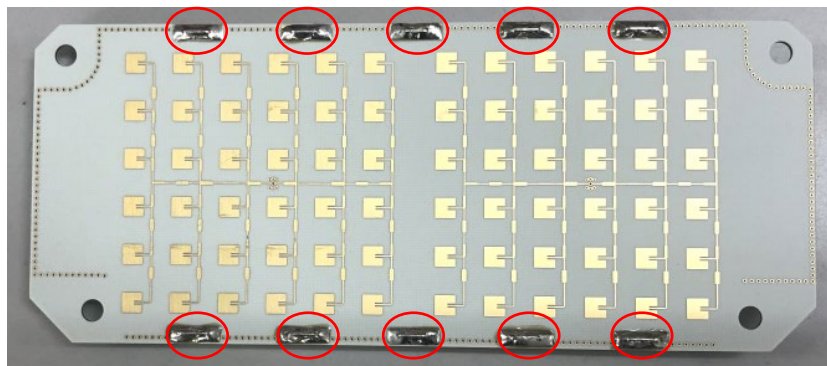
Product Completion State (Antenna Side)
